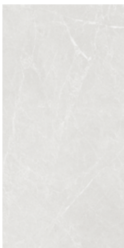
MERCURY
